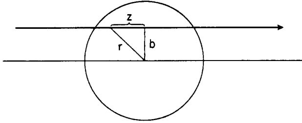
Fig. 1. Straight-line trajectory at impact parameter b , for evaluating Glauber phase shift.
