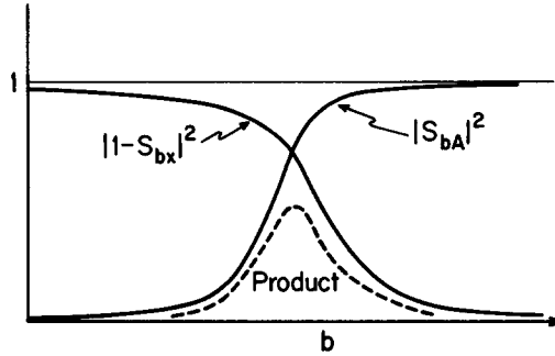
Fig. 2. Schematic representation of the absorption factors of eq. (4.17), indicating how they limit the integration to the surface region of the target.
